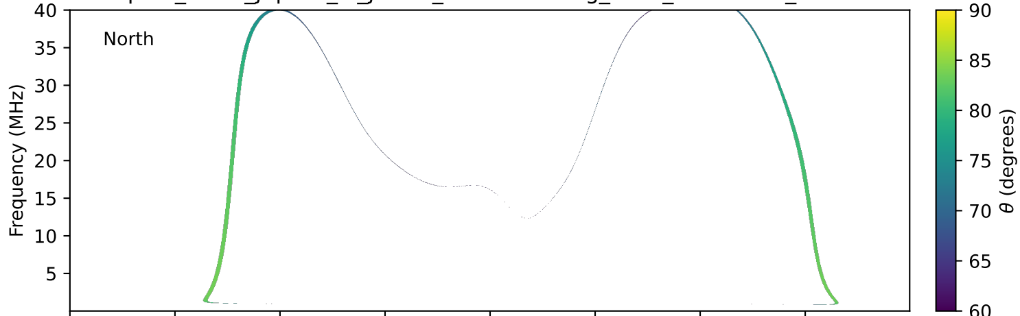
expres_earth_jupiter_io_jrm33_lossc-wid1deg_3kev_20190509_v11.cdf
