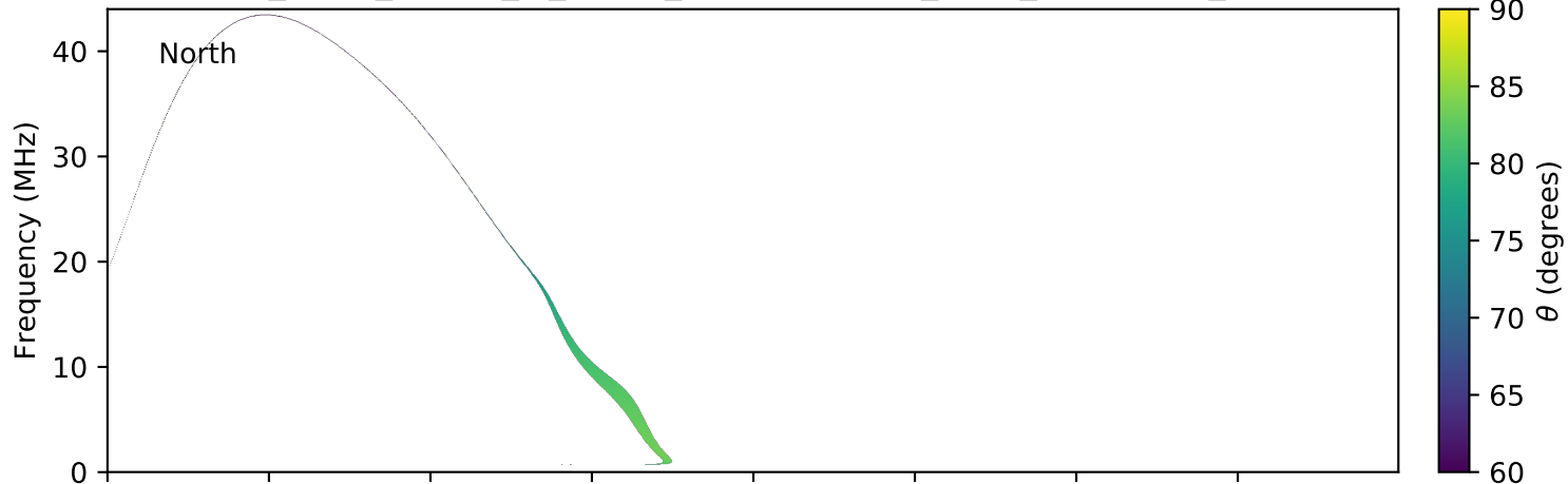
expres_earth_jupiter_io_jrm09_lossc-wid1deg_3kev_20190529_v01.cdf
