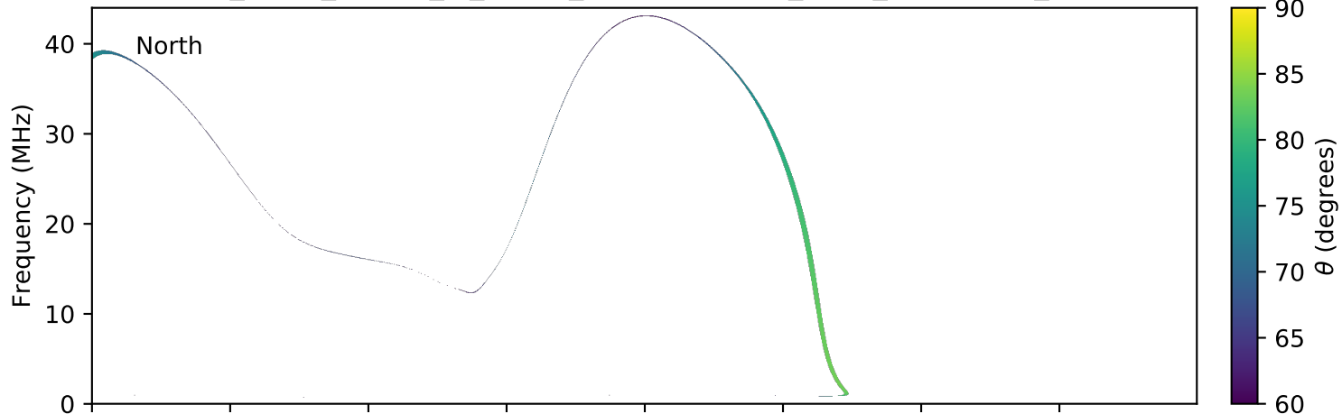
expres_earth_jupiter_io_jrm09_lossc-wid1deg_3kev_20190527_v01.cdf
