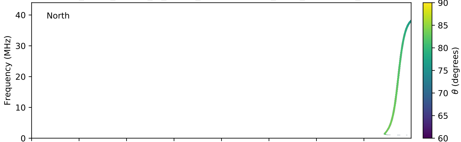
expres_earth_jupiter_io_jrm09_lossc-wid1deg_3kev_20190526_v01.cdf
