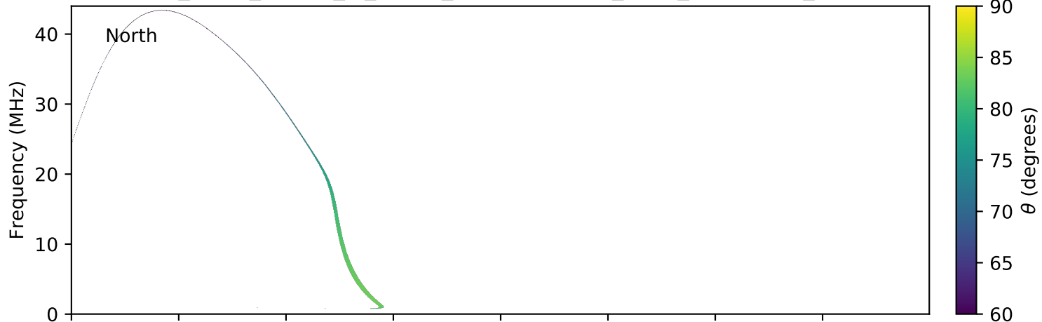
expres_earth_jupiter_io_jrm09_lossc-wid1deg_3kev_20190522_v01.cdf
