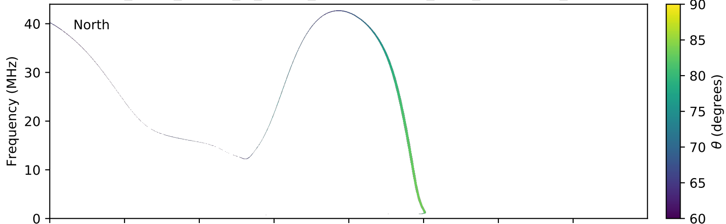
expres_earth_jupiter_io_jrm09_lossc-wid1deg_3kev_20190520_v01.cdf
