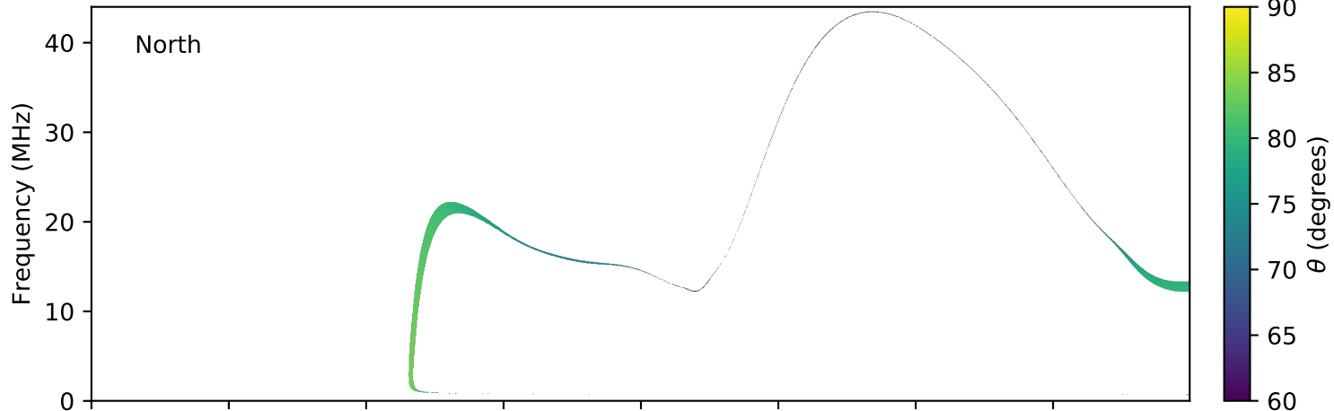
expres_earth_jupiter_io_jrm09_lossc-wid1deg_3kev_20190516_v01.cdf
