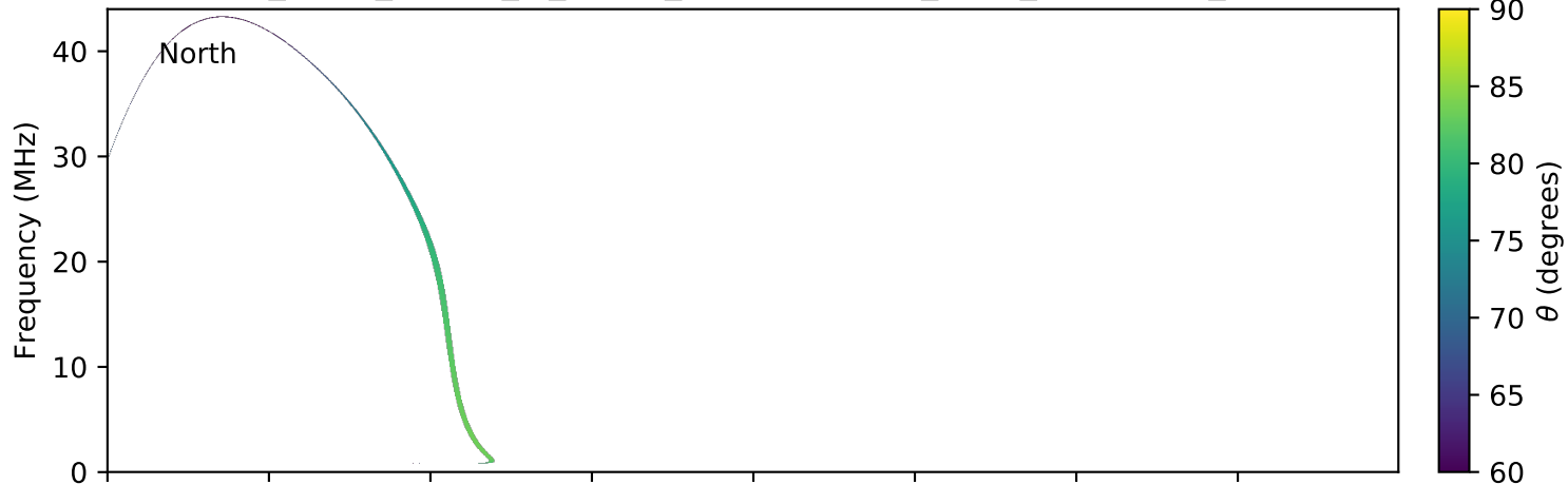
expres_earth_jupiter_io_jrm09_lossc-wid1deg_3kev_20190515_v01.cdf
