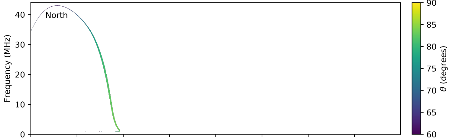
expres_earth_jupiter_io_jrm09_lossc-wid1deg_3kev_20190508_v01.cdf
