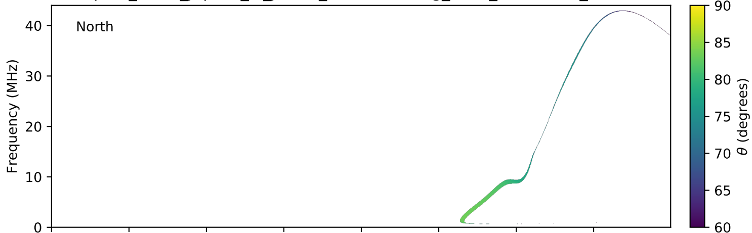
expres_earth_jupiter_io_jrm09_lossc-wid1deg_3kev_20190505_v01.cdf
