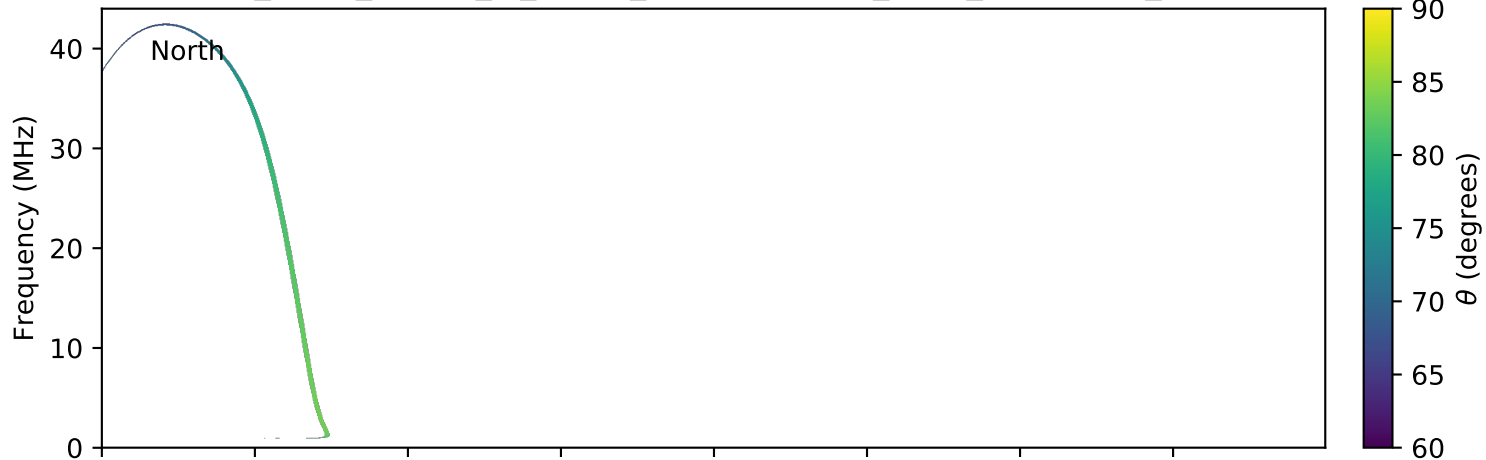
expres_earth_jupiter_io_jrm09_lossc-wid1deg_3kev_20190501_v01.cdf
