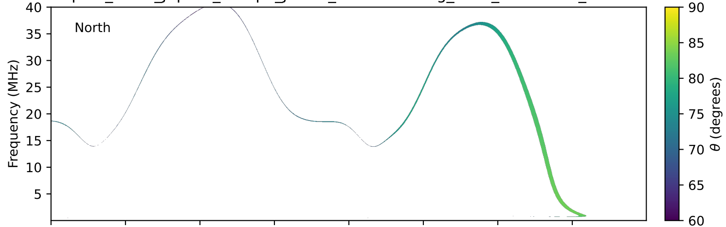
expres_earth_jupiter_europa_jrm33_lossc-wid1deg_3kev_20190514_v11.cdf
