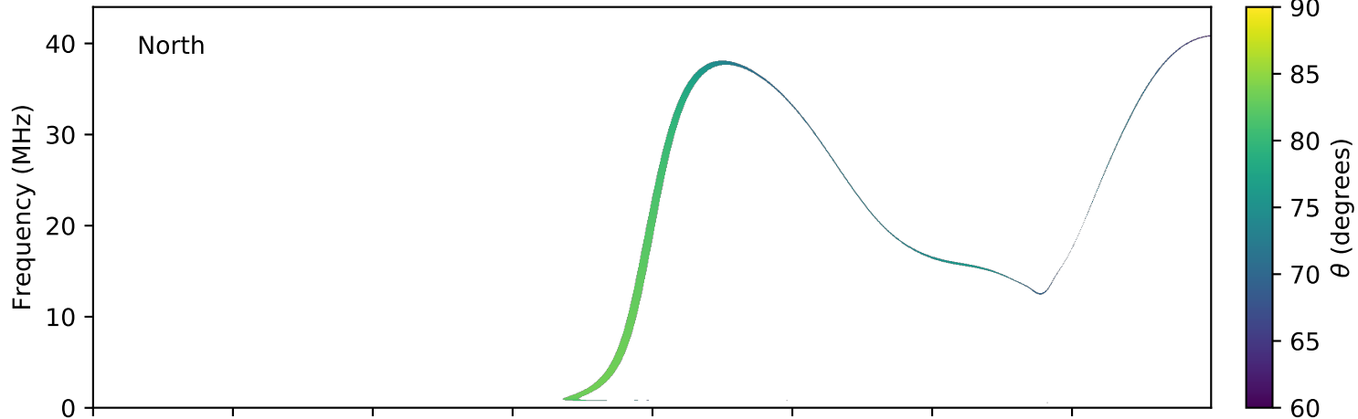
expres_earth_jupiter_europa_jrm09_lossc-wid1deg_3kev_20190531_v01.cdf
