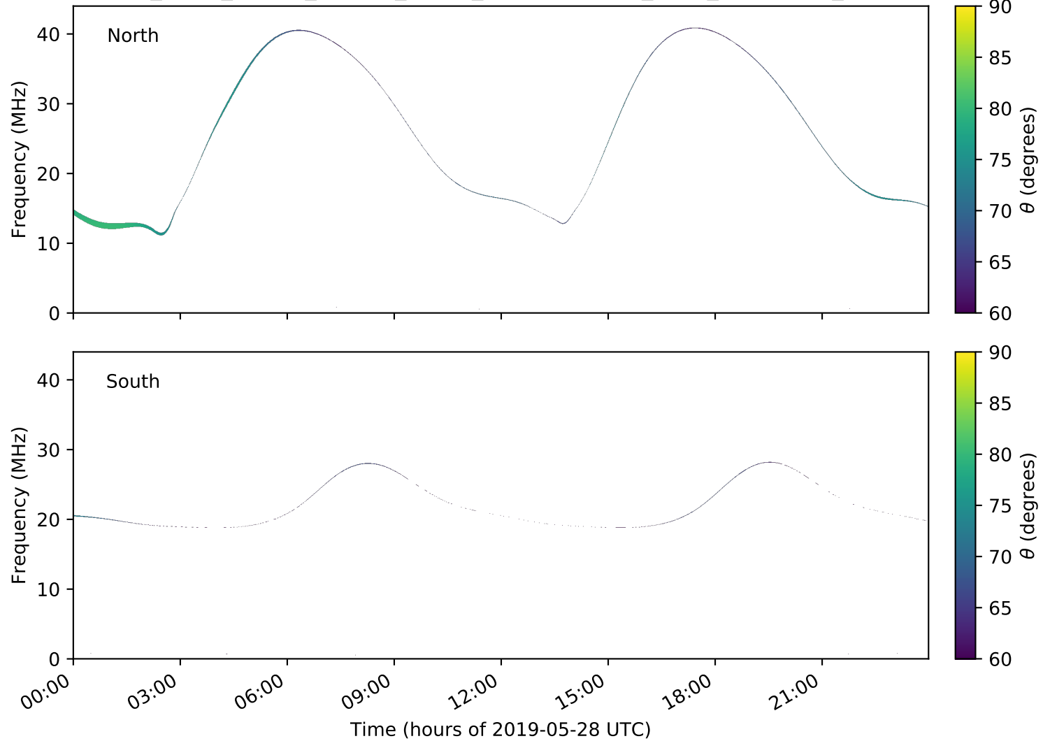
expres_earth_jupiter_europa_jrm09_lossc-wid1deg_3kev_20190528_v01.cdf
