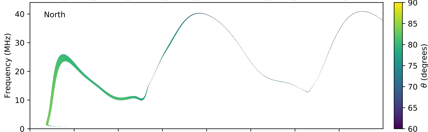
expres_earth_jupiter_europa_jrm09_lossc-wid1deg_3kev_20190510_v01.cdf
