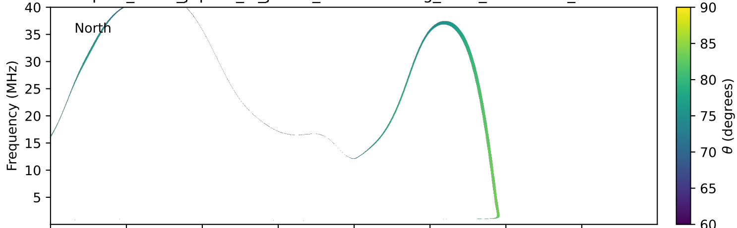
expres_earth_jupiter_io_jrm33_lossc-wid1deg_3kev_20190418_v11.cdf
