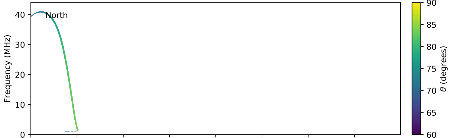
expres_earth_jupiter_io_jrm09_lossc-wid1deg_3kev_20190424_v01.cdf
