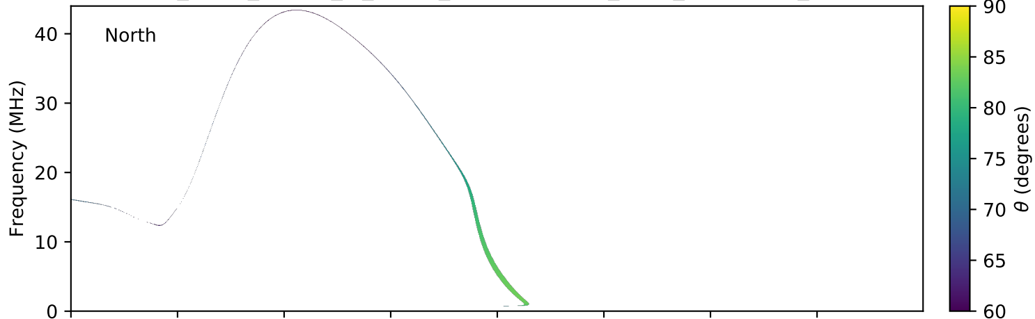
expres_earth_jupiter_io_jrm09_lossc-wid1deg_3kev_20190420_v01.cdf
