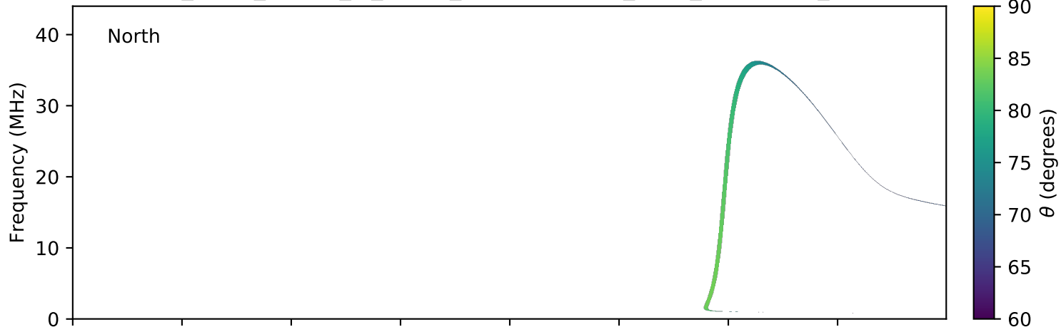
expres_earth_jupiter_io_jrm09_lossc-wid1deg_3kev_20190412_v01.cdf
