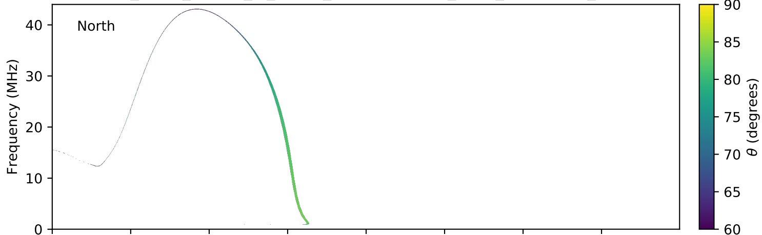
expres_earth_jupiter_io_jrm09_lossc-wid1deg_3kev_20190406_v01.cdf
