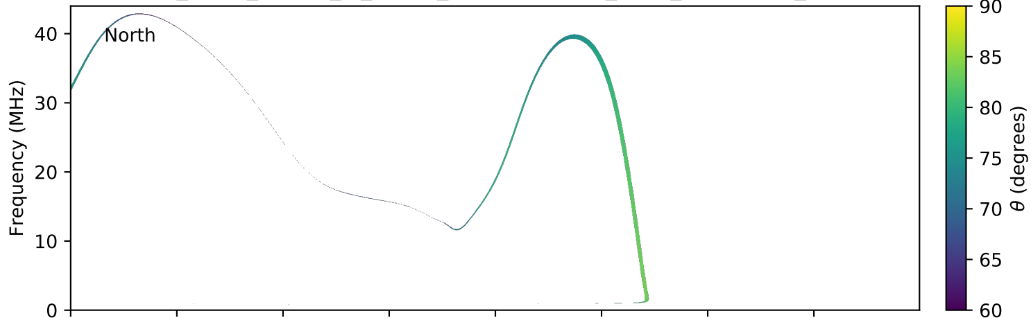
expres_earth_jupiter_io_jrm09_lossc-wid1deg_3kev_20190404_v01.cdf
