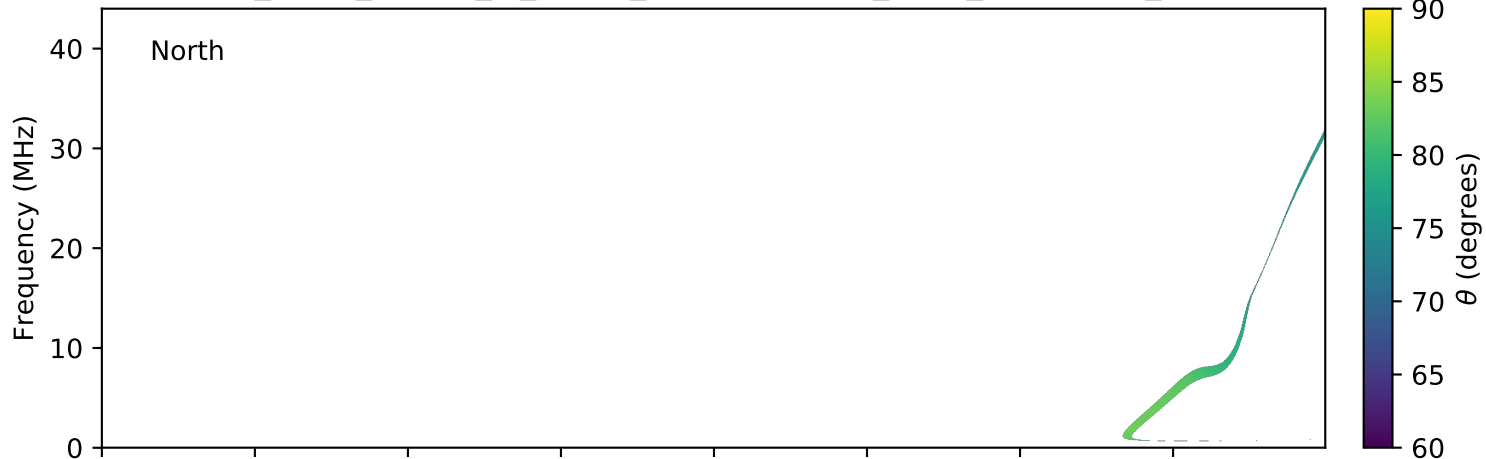
expres_earth_jupiter_io_jrm09_lossc-wid1deg_3kev_20190403_v01.cdf
