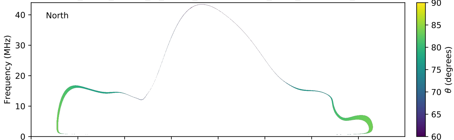
expres_earth_jupiter_io_jrm09_lossc-wid1deg_3kev_20190402_v01.cdf
