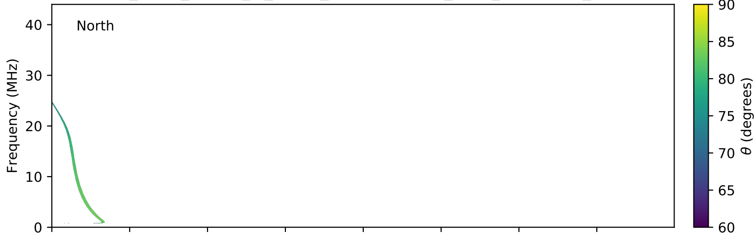
expres_earth_jupiter_io_jrm09_lossc-wid1deg_3kev_20190401_v01.cdf
