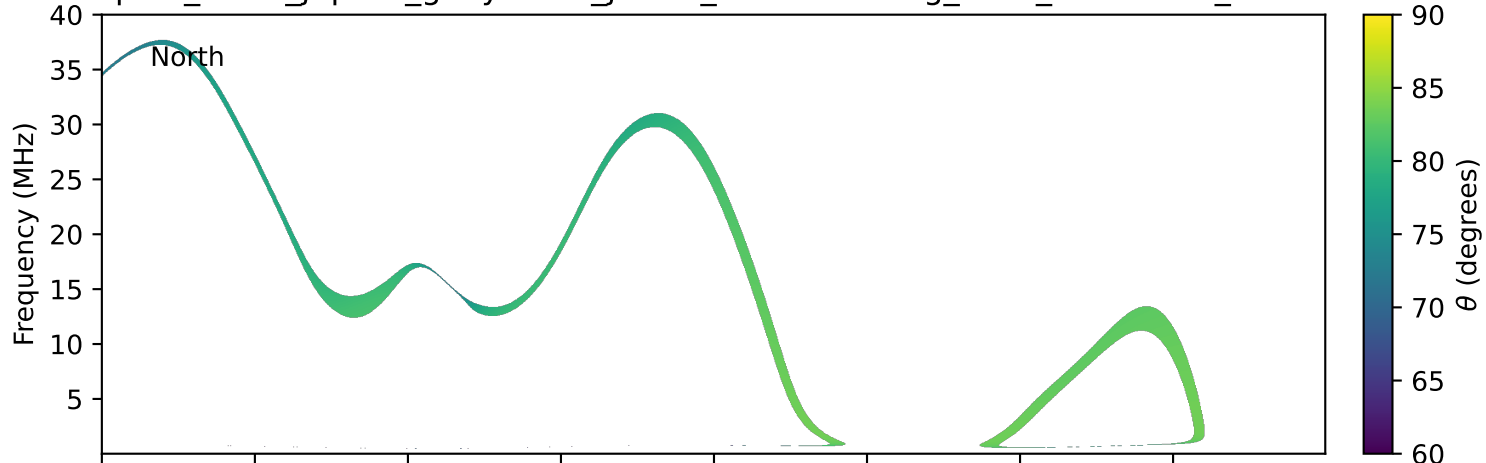
expres_earth_jupiter_ganymede_jrm33_lossc-wid1deg_3kev_20190424_v11.cdf
