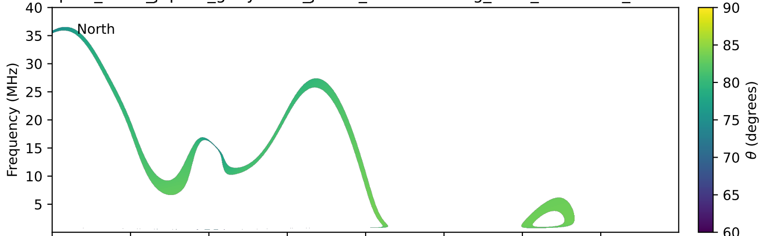
expres_earth_jupiter_ganymede_jrm33_lossc-wid1deg_3kev_20190417_v11.cdf
