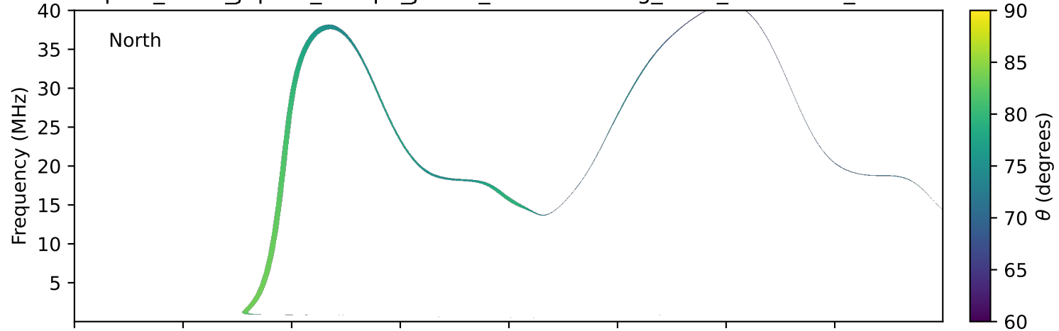
expres_earth_jupiter_europa_jrm33_lossc-wid1deg_3kev_20190422_v11.cdf
