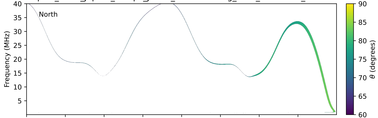
expres_earth_jupiter_europa_jrm33_lossc-wid1deg_3kev_20190412_v11.cdf
