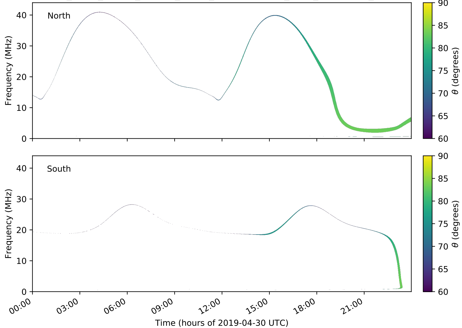
expres_earth_jupiter_europa_jrm09_lossc-wid1deg_3kev_20190430_v01.cdf
