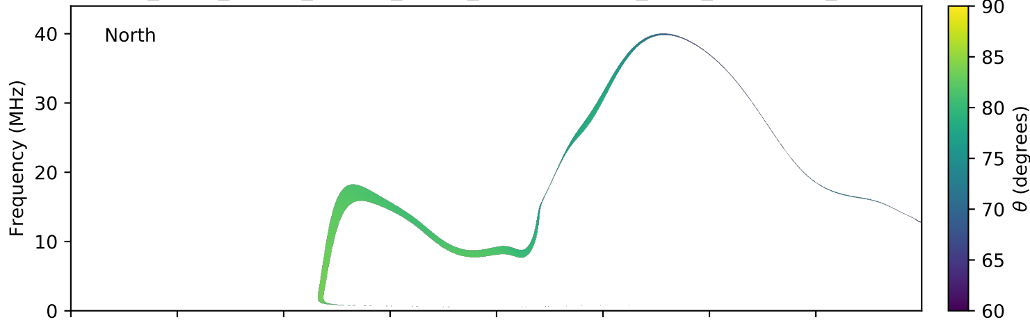
expres_earth_jupiter_europa_jrm09_lossc-wid1deg_3kev_20190422_v01.cdf
