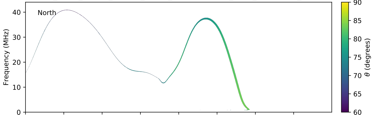
expres_earth_jupiter_europa_jrm09_lossc-wid1deg_3kev_20190416_v01.cdf
