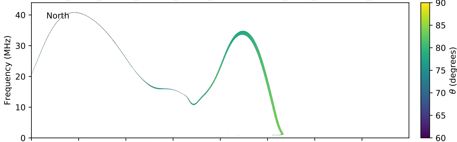
expres_earth_jupiter_europa_jrm09_lossc-wid1deg_3kev_20190409_v01.cdf
