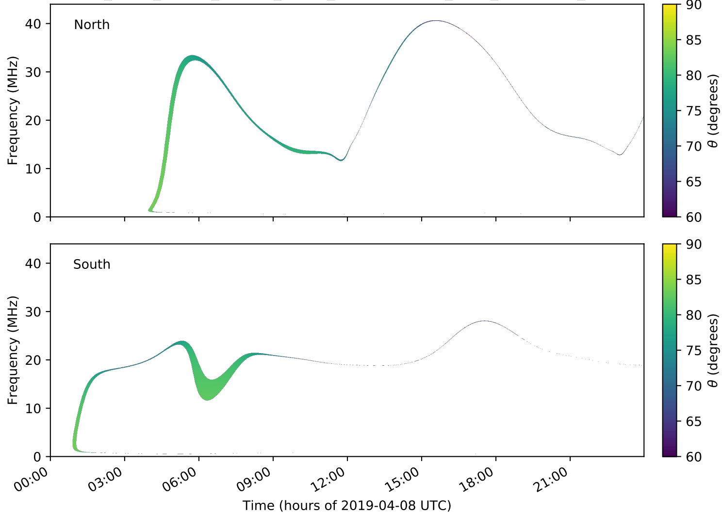
expres_earth_jupiter_europa_jrm09_lossc-wid1deg_3kev_20190408_v01.cdf
