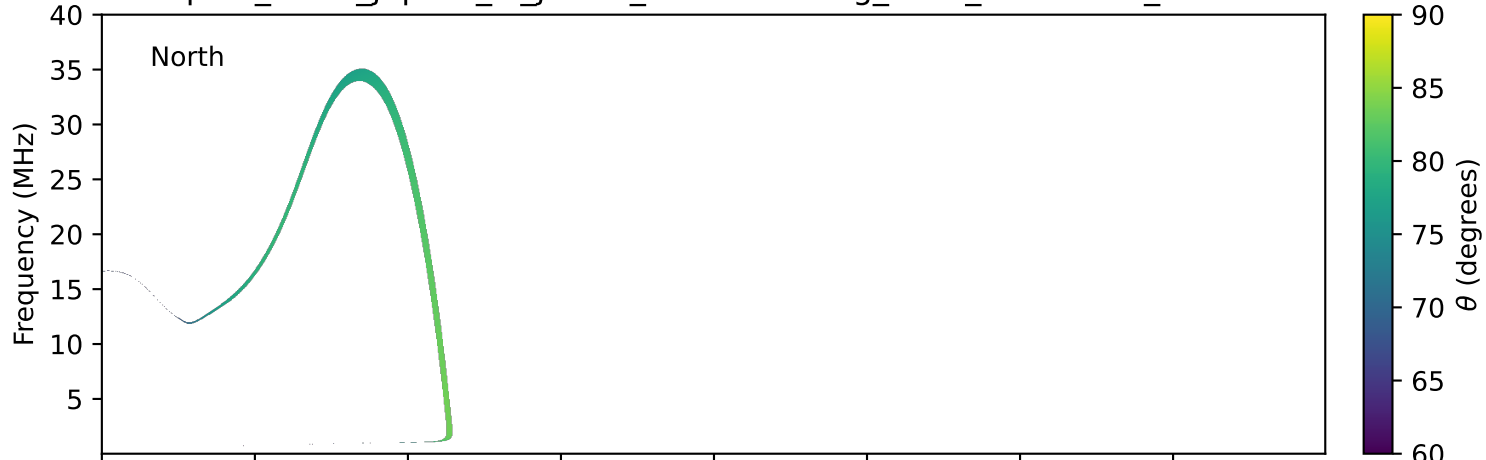
expres_earth_jupiter_io_jrm33_lossc-wid1deg_3kev_20190330_v11.cdf
