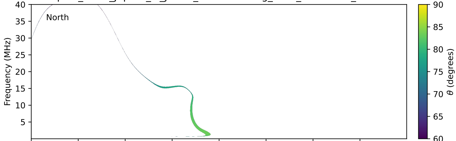
expres_earth_jupiter_io_jrm33_lossc-wid1deg_3kev_20190328_v11.cdf
