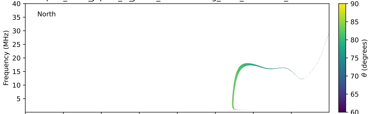
expres_earth_jupiter_io_jrm33_lossc-wid1deg_3kev_20190327_v11.cdf
