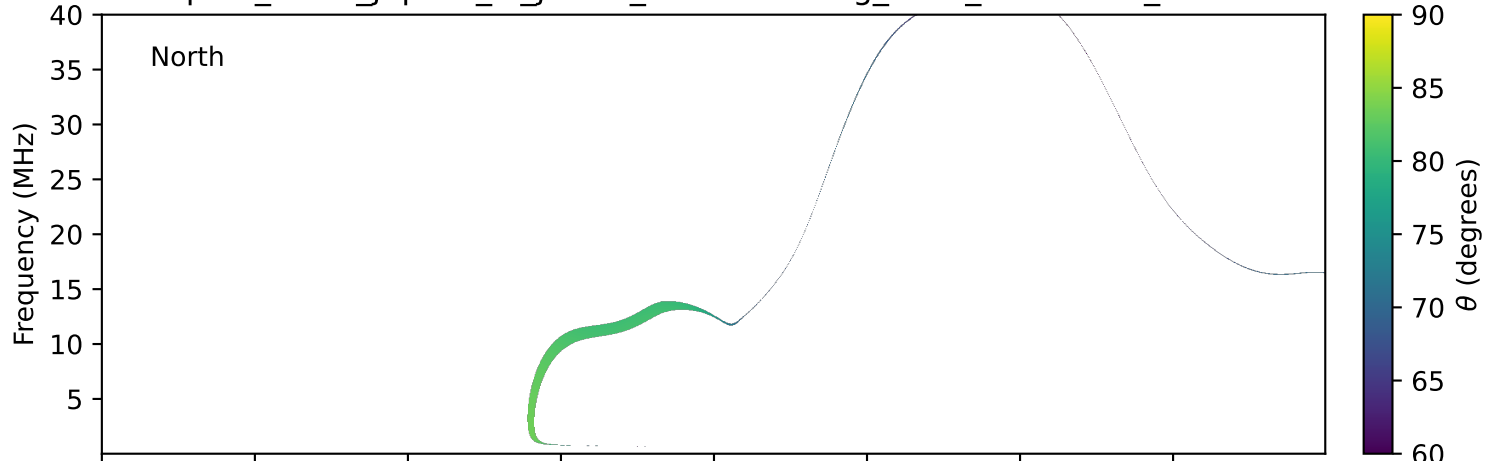
expres_earth_jupiter_io_jrm33_lossc-wid1deg_3kev_20190322_v11.cdf
