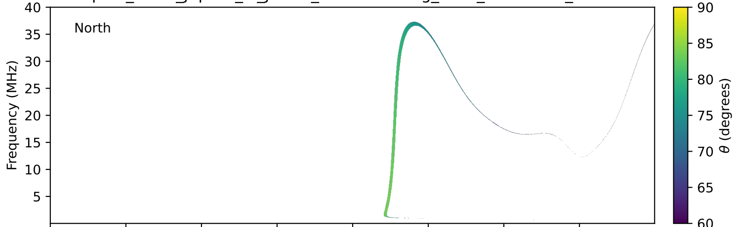
expres_earth_jupiter_io_jrm33_lossc-wid1deg_3kev_20190313_v11.cdf
