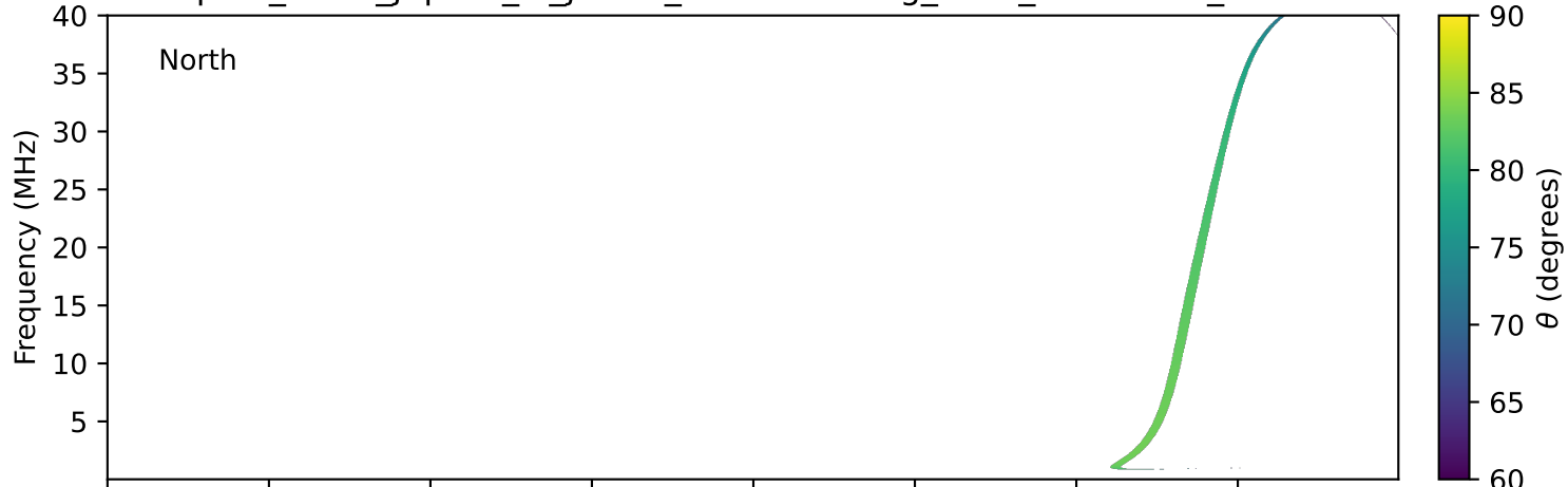
expres_earth_jupiter_io_jrm33_lossc-wid1deg_3kev_20190311_v11.cdf
