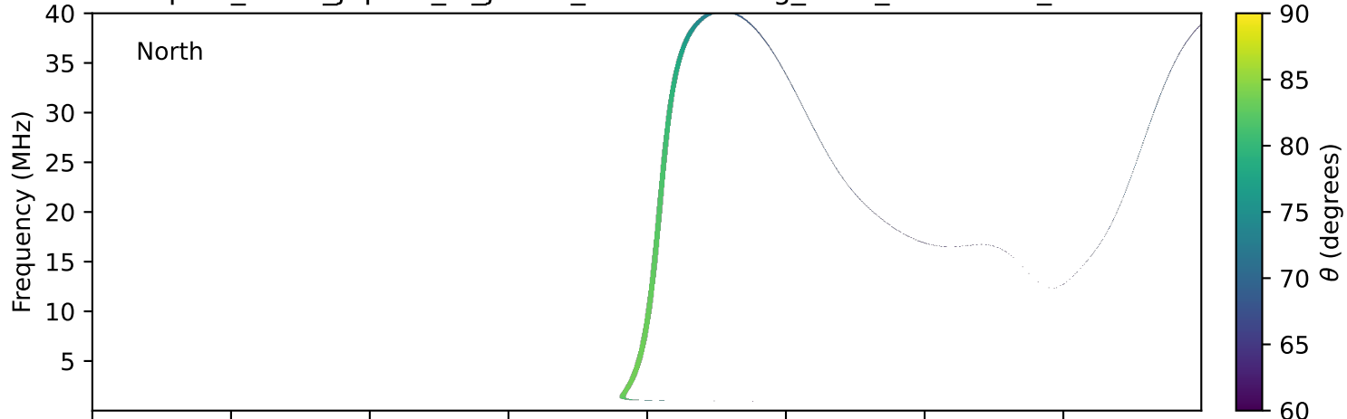
expres_earth_jupiter_io_jrm33_lossc-wid1deg_3kev_20190306_v11.cdf
