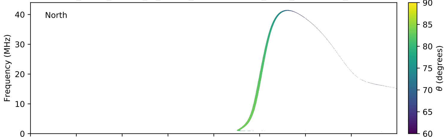
expres_earth_jupiter_io_jrm09_lossc-wid1deg_3kev_20190329_v01.cdf
