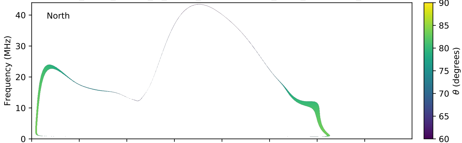
expres_earth_jupiter_io_jrm09_lossc-wid1deg_3kev_20190326_v01.cdf
