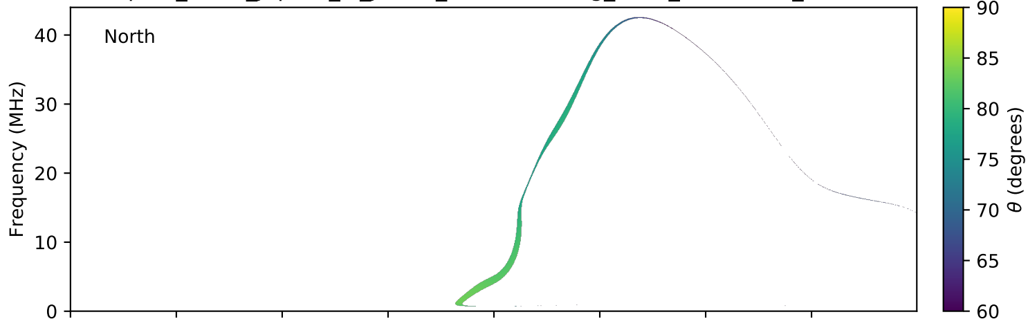
expres_earth_jupiter_io_jrm09_lossc-wid1deg_3kev_20190322_v01.cdf
