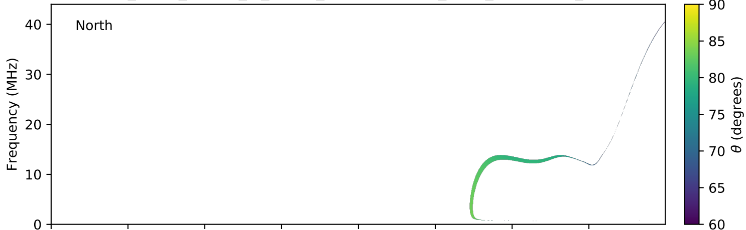
expres_earth_jupiter_io_jrm09_lossc-wid1deg_3kev_20190320_v01.cdf
