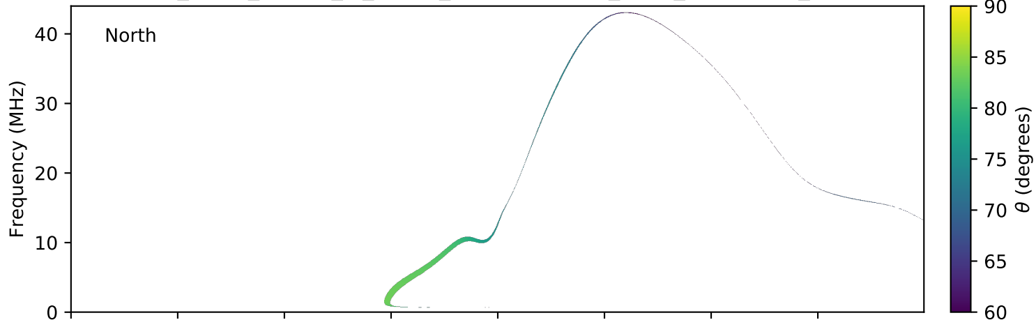
expres_earth_jupiter_io_jrm09_lossc-wid1deg_3kev_20190315_v01.cdf
