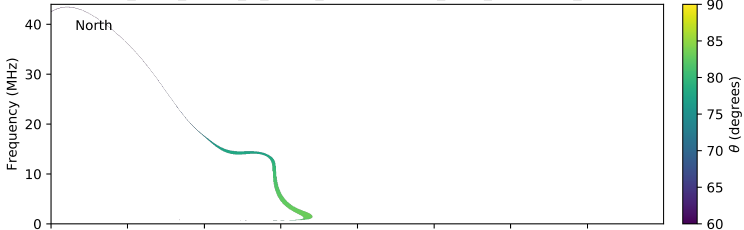
expres_earth_jupiter_io_jrm09_lossc-wid1deg_3kev_20190314_v01.cdf
