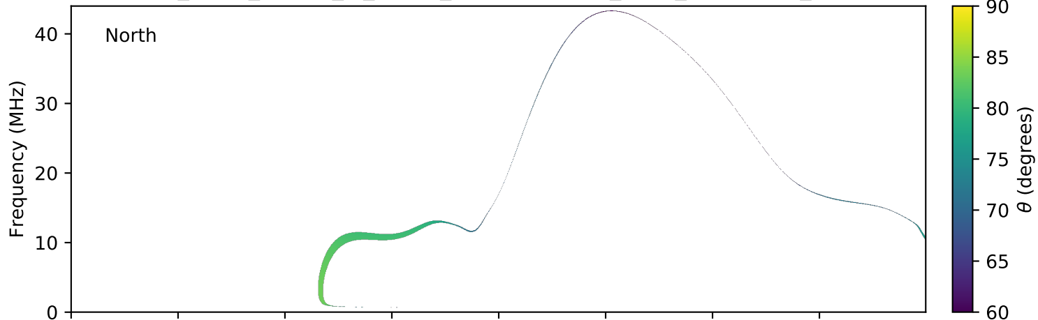
expres_earth_jupiter_io_jrm09_lossc-wid1deg_3kev_20190308_v01.cdf
