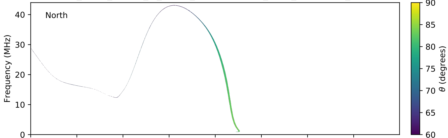
expres_earth_jupiter_io_jrm09_lossc-wid1deg_3kev_20190305_v01.cdf
