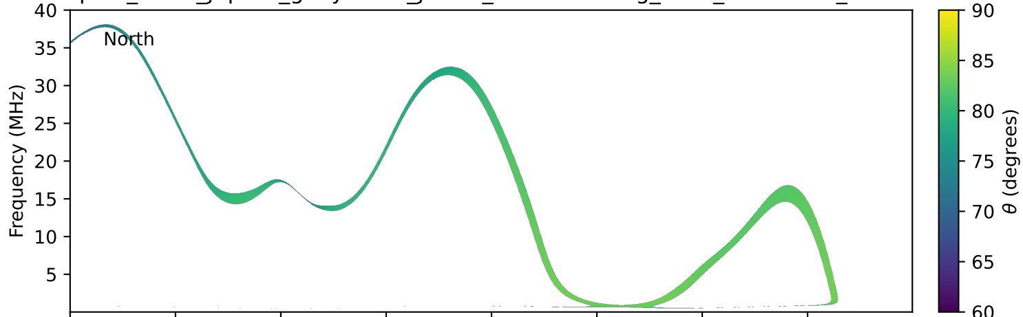
expres_earth_jupiter_ganymede_jrm33_lossc-wid1deg_3kev_20190312_v11.cdf
