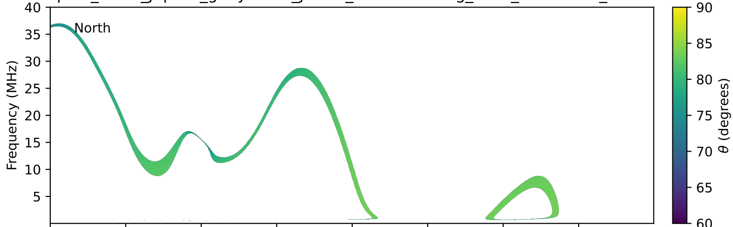
expres_earth_jupiter_ganymede_jrm33_lossc-wid1deg_3kev_20190305_v11.cdf
